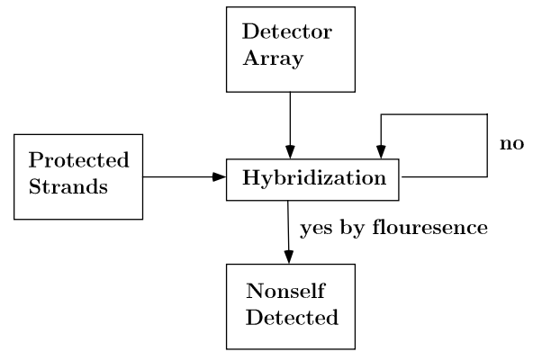
Figure 1: Algorithm for Censoring (after [4]).
