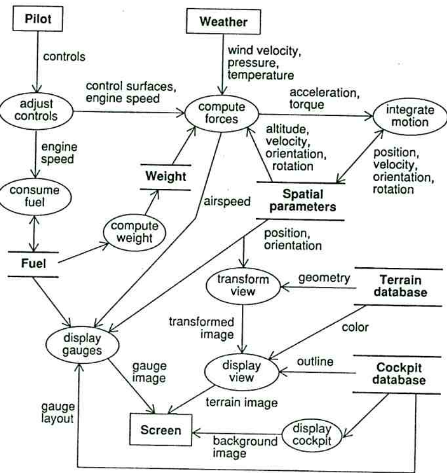
Functional model of flight simulator
